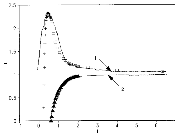
Figure 2. Dependence of tip current (normalized to i_{T,\infty} ) on relative tip displacement (normalized to tip radius) over a conductive n- \text{TiO}_2 substrate ( E_s = -0.7 \text{ V} vs SCE), curve 1, and an insulating n- \text{TiO}_2 substrate ( E_s = 0.0 \text{ V} vs SCE), curve 2, in a solution containing 2 mM \text{Cp}_2\text{FeTMA}^+ and 1.0 M \text{NaNO}_3 . The tip was biased at 0.60 V vs SCE. The tip moved to the substrate surface at a rate of 38 \text{ \AA/s} . Solid curves are experimental data and symbols are theory. ( \square ) Simulated data for conducting substrate; (+) calculated data based on eq 3; ( \Delta ) simulated data for insulating substrate. Fitting parameters: a = 45 \text{ nm} , a_0 = 67 \text{ nm} , l = 28 \text{ nm} , and D = 5.0 \times 10^{-6} \text{ cm}^2/\text{s} . Experimental i_{T,\infty} is equal to 9.0 pA.
